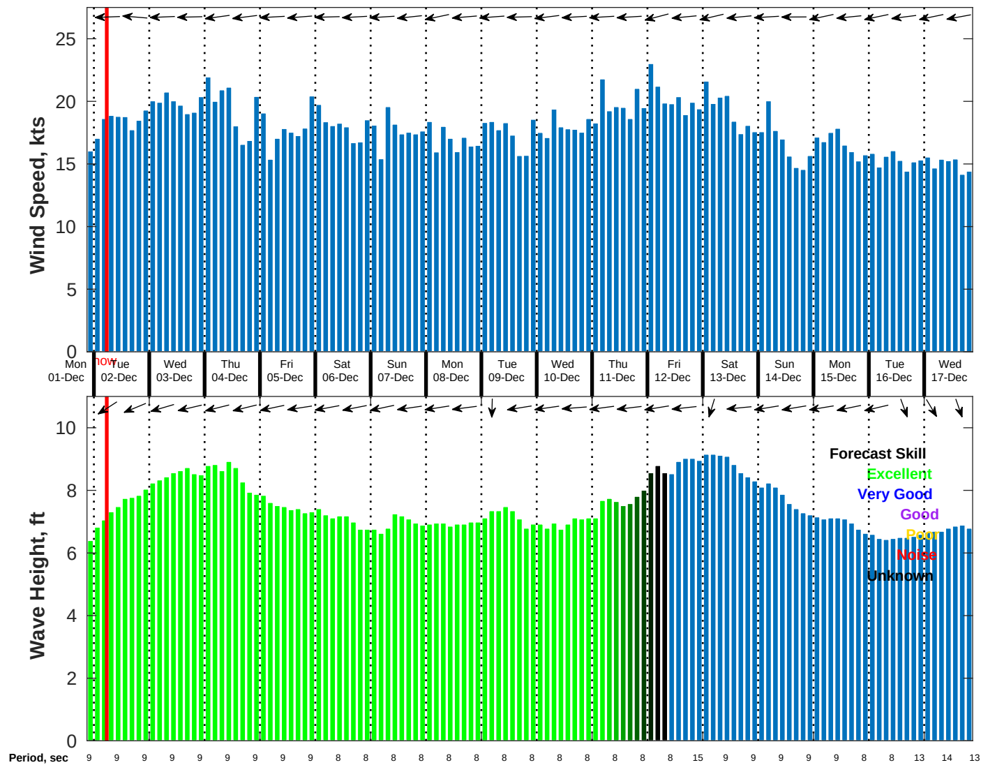
Wind & Wave Forecast for NDBC 41040 from 01-Dec-2025 21:00:00 to 17-Dec-2025 21:00:00
