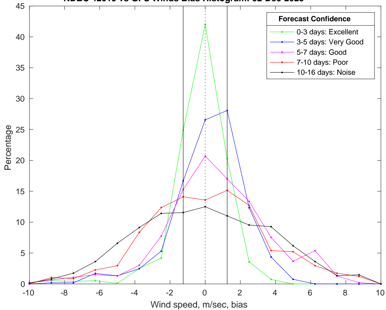
NDBC 42019 vs GFS Winds Bias Histogram: 02-Dec-2025
