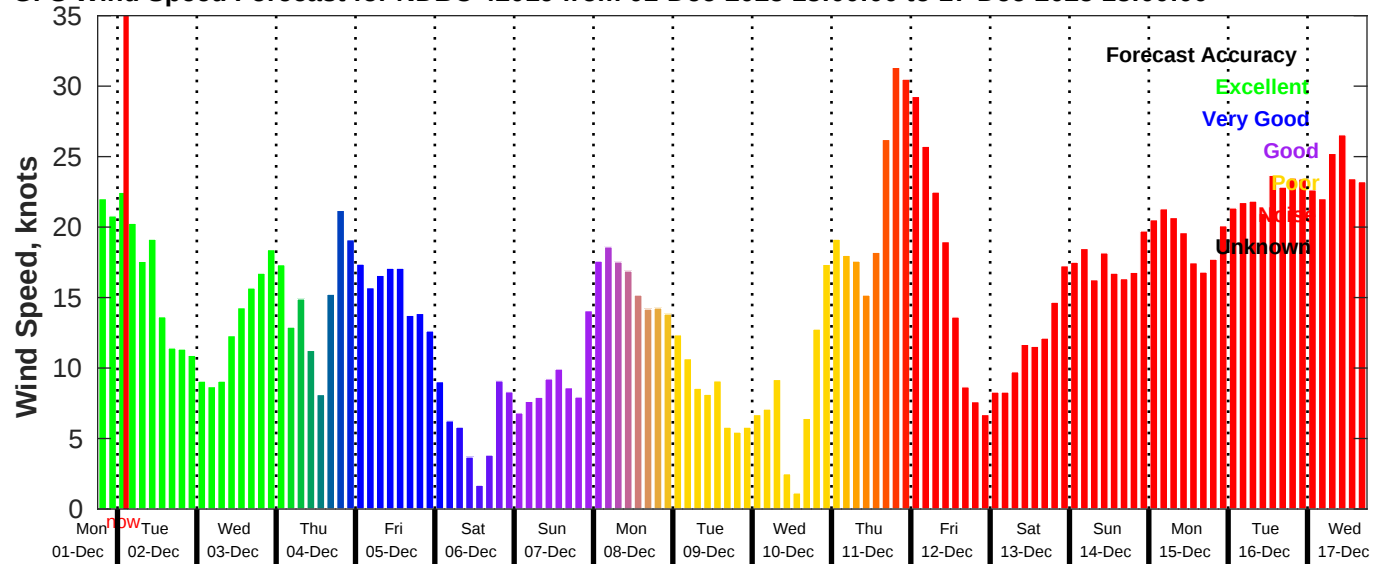
GFS Wind Speed Forecast for NDBC 42019 from 01-Dec-2025 18:00:00 to 17-Dec-2025 18:00:00
