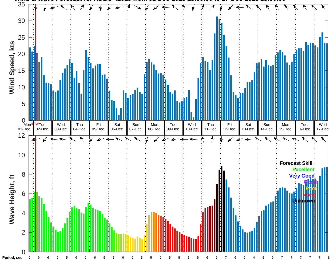
Wind & Wave Forecast for NDBC 42019 from 01-Dec-2025 18:00:00 to 17-Dec-2025 18:00:00
