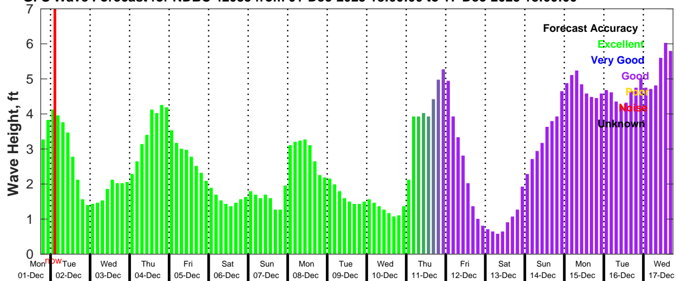
GFS Wave Forecast for NDBC 42035 from 01-Dec-2025 18:00:00 to 17-Dec-2025 18:00:00
