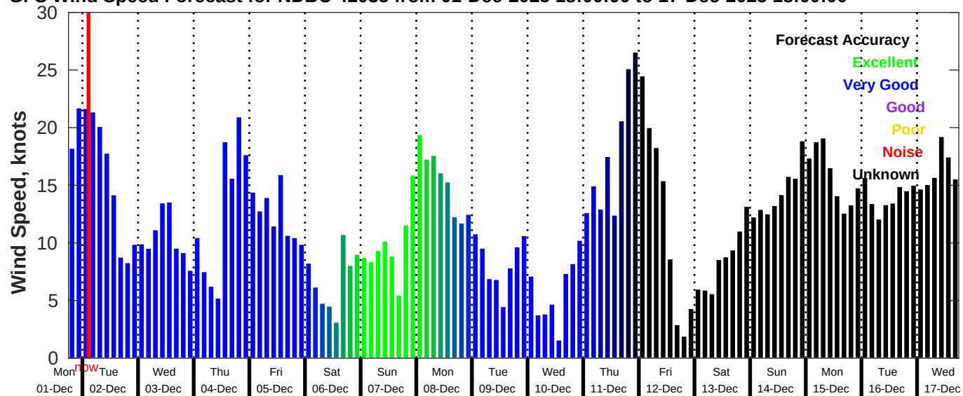
GFS Wind Speed Forecast for NDBC 42035 from 01-Dec-2025 18:00:00 to 17-Dec-2025 18:00:00
