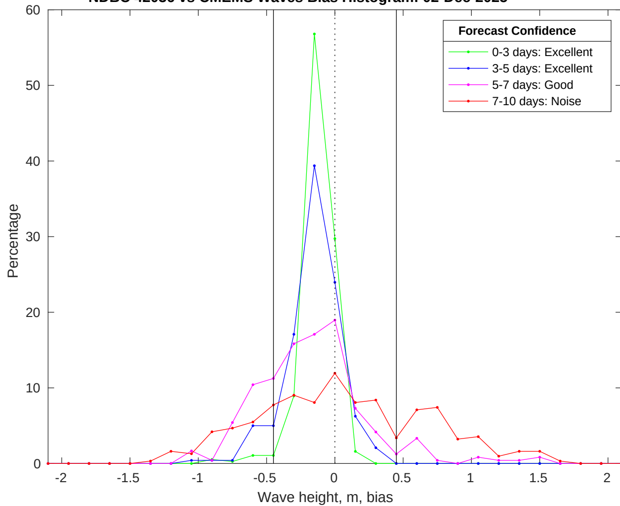
NDBC 42036 vs CMEMS Waves Bias Histogram: 02-Dec-2025
