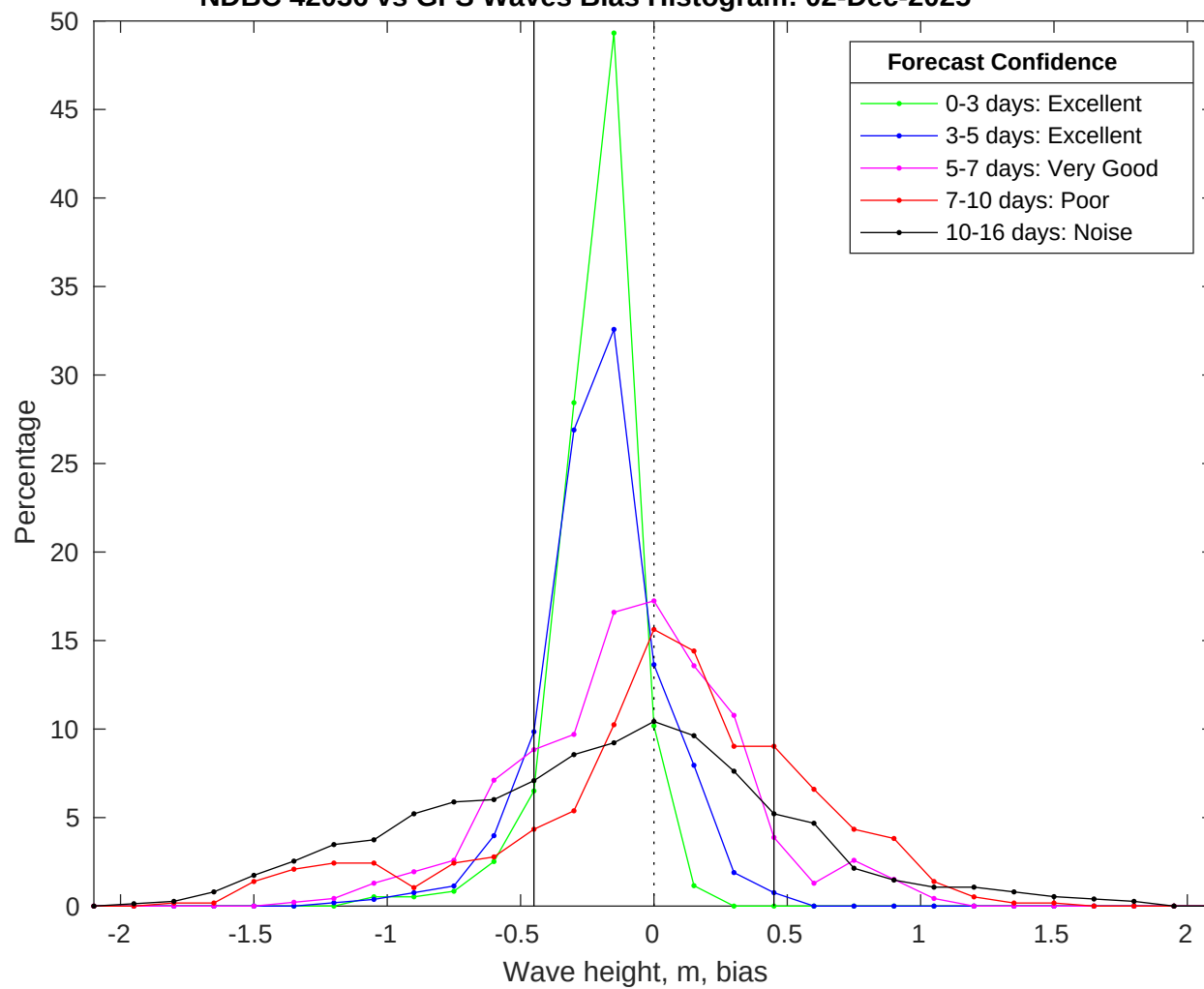
NDBC 42036 vs GFS Waves Bias Histogram: 02-Dec-2025
