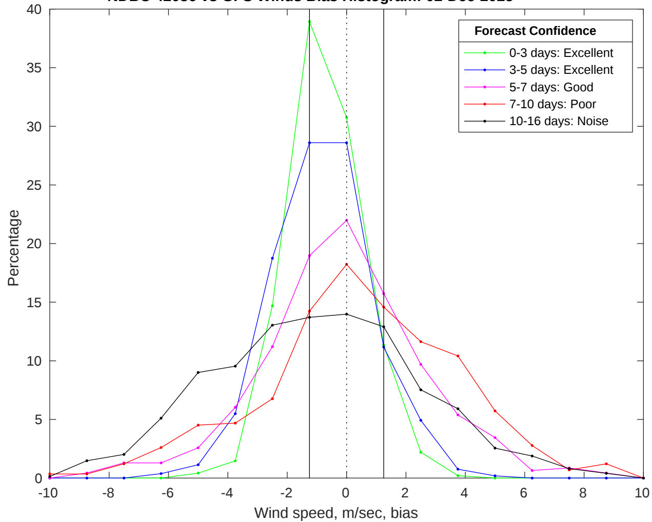
NDBC 42036 vs GFS Winds Bias Histogram: 02-Dec-2025
