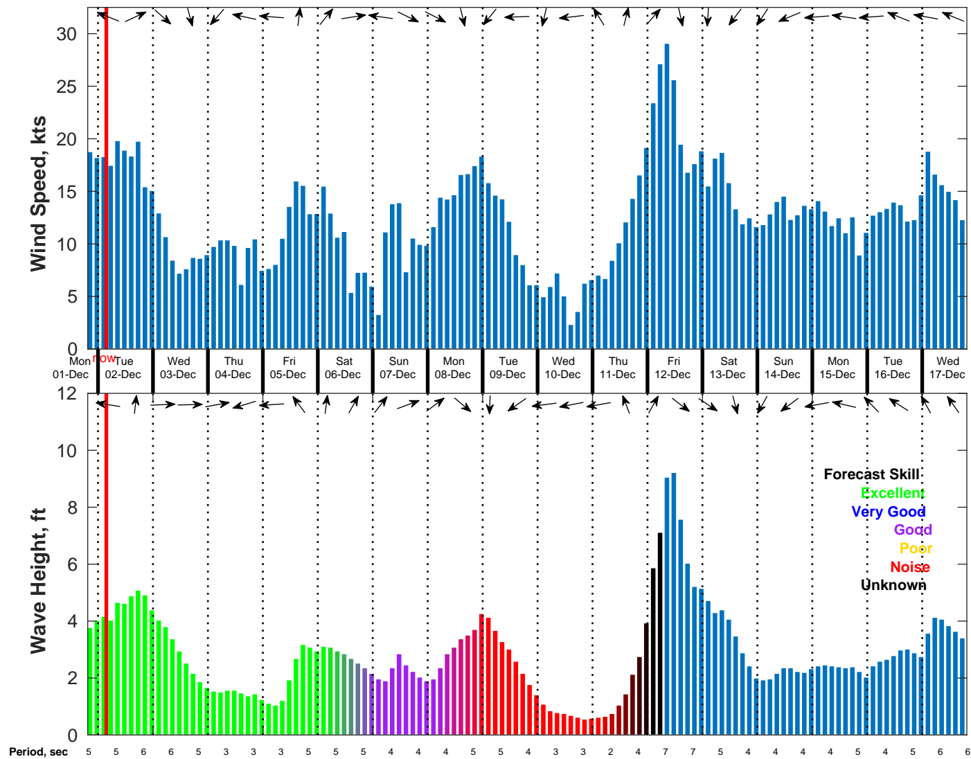
Wind & Wave Forecast for NDBC 42036 from 01-Dec-2025 19:00:00 to 17-Dec-2025 19:00:00
