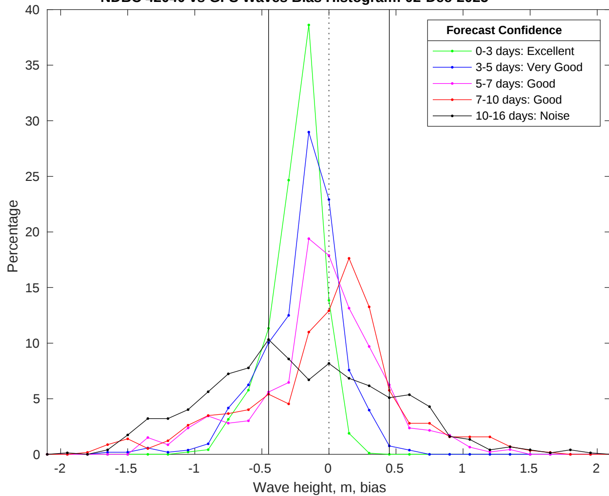
NDBC 42040 vs GFS Waves Bias Histogram: 02-Dec-2025
