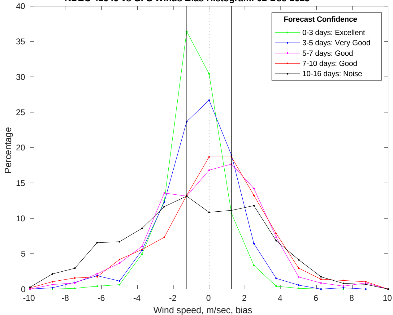
NDBC 42040 vs GFS Winds Bias Histogram: 02-Dec-2025
