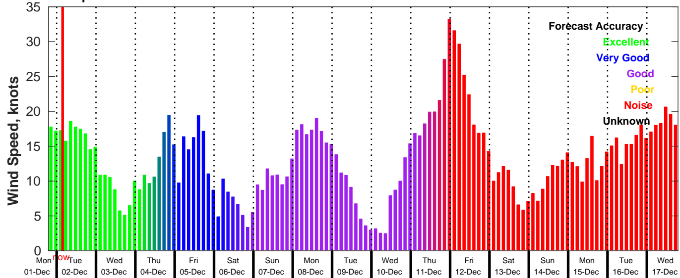
GFS Wind Speed Forecast for NDBC 42040 from 01-Dec-2025 19:00:00 to 17-Dec-2025 19:00:00
