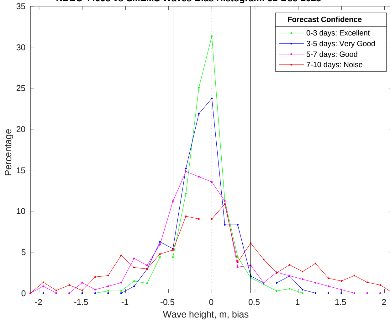
NDBC 44008 vs CMEMS Waves Bias Histogram: 02-Dec-2025
