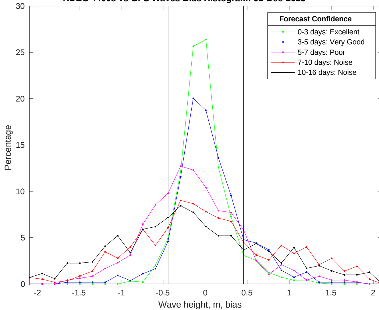
NDBC 44008 vs GFS Waves Bias Histogram: 02-Dec-2025
