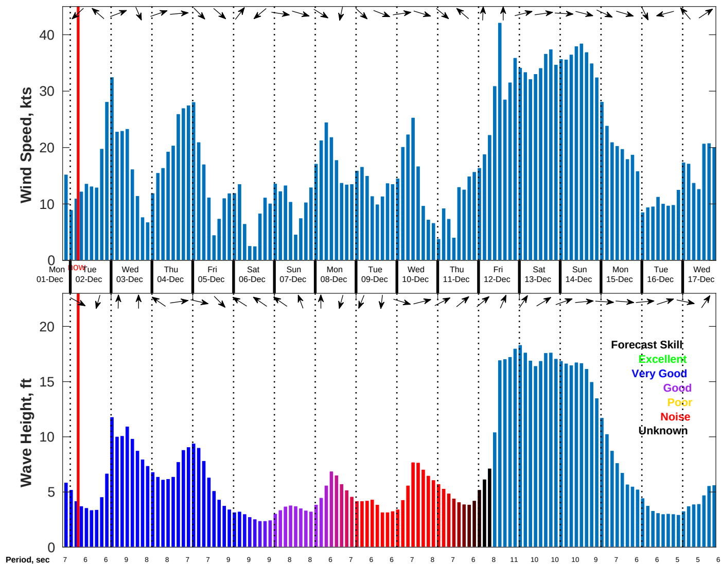
Wind & Wave Forecast for NDBC 44008 from 01-Dec-2025 20:00:00 to 17-Dec-2025 20:00:00
