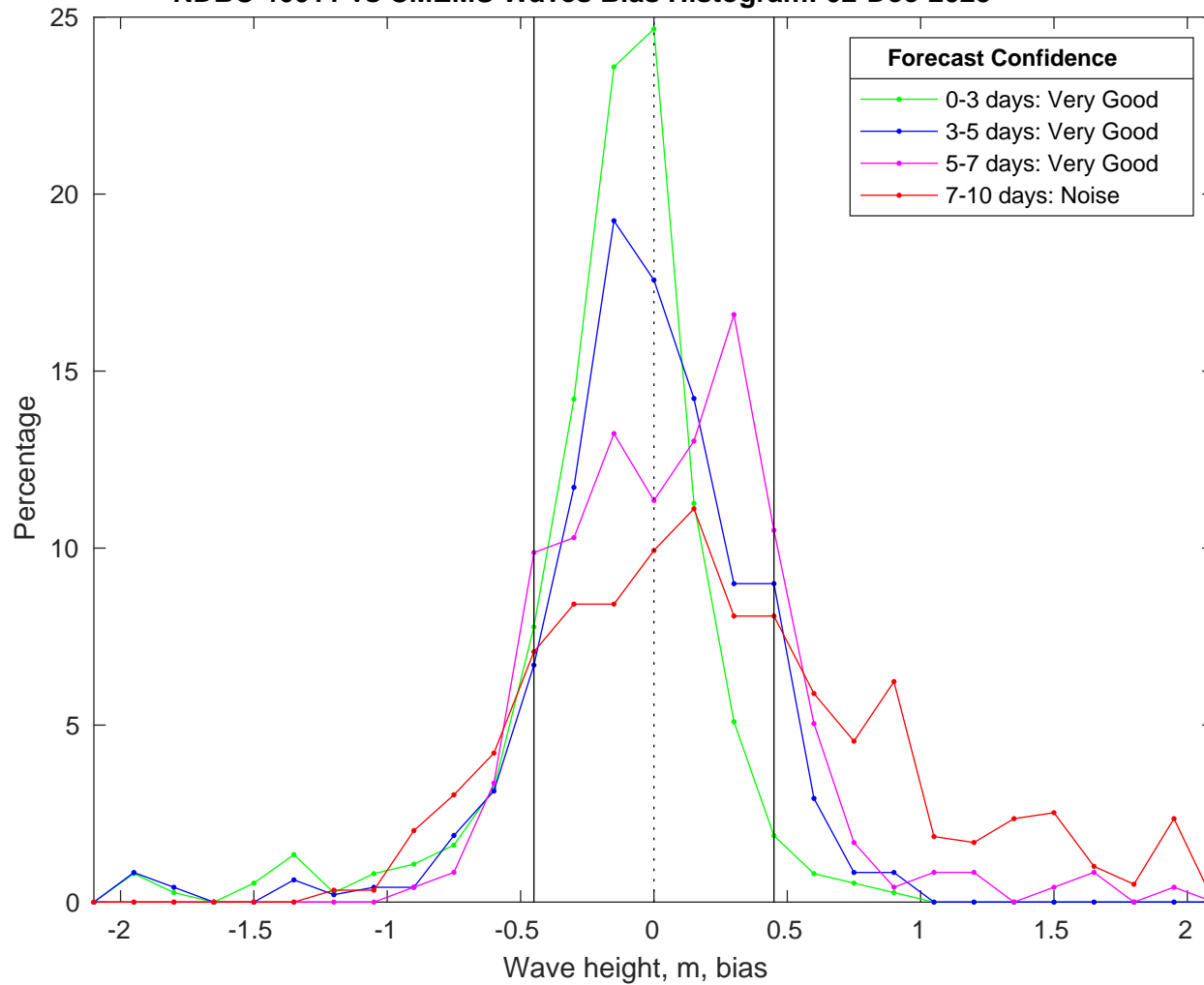
NDBC 46011 vs CMEMS Waves Bias Histogram: 02-Dec-2025
