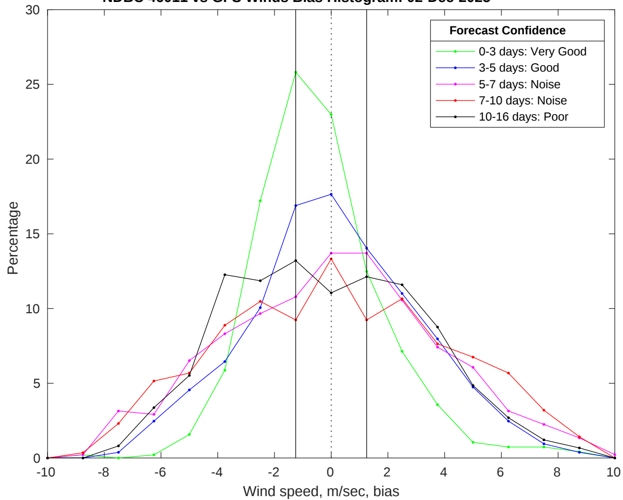
NDBC 46011 vs GFS Winds Bias Histogram: 02-Dec-2025
