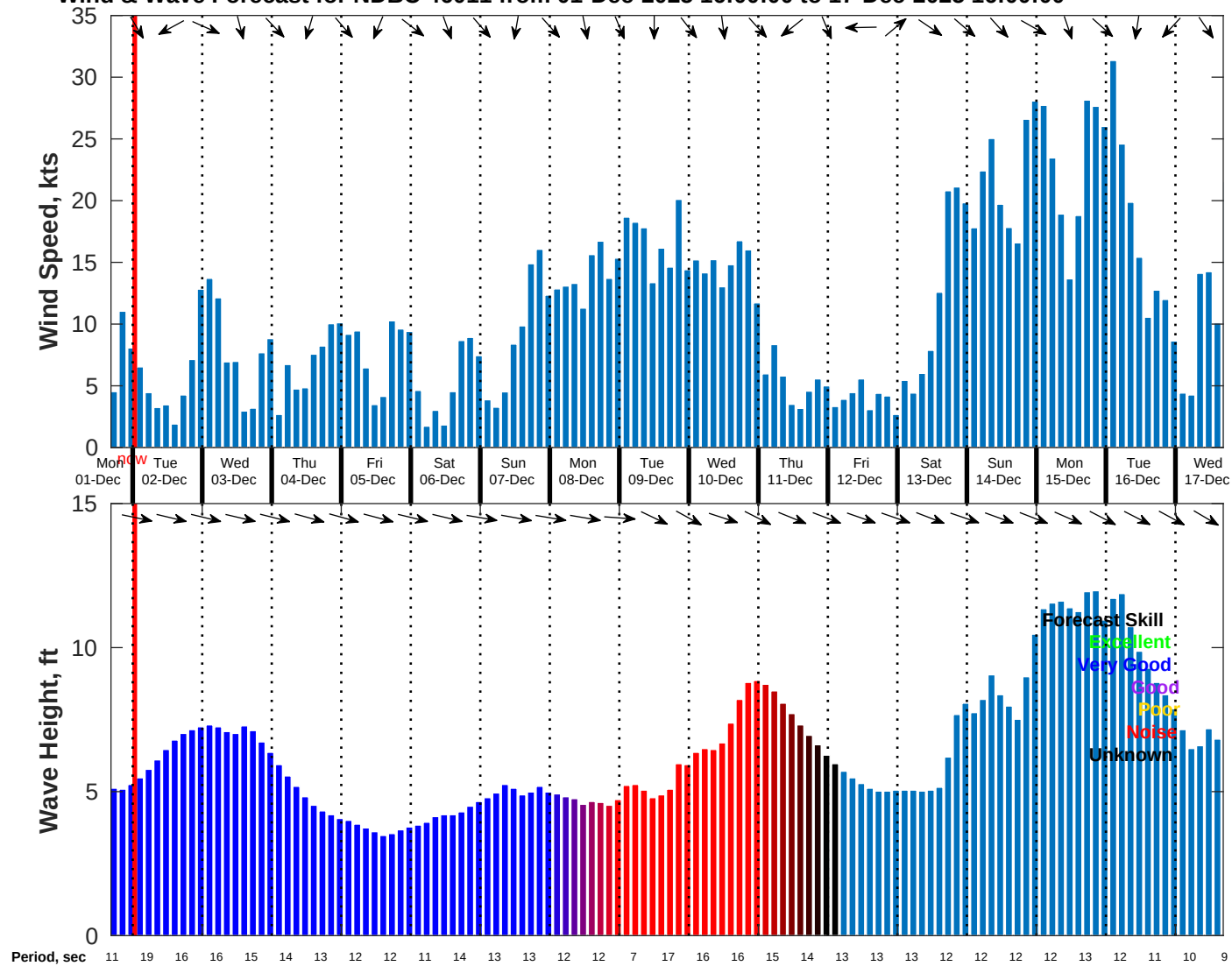
Wind & Wave Forecast for NDBC 46011 from 01-Dec-2025 16:00:00 to 17-Dec-2025 16:00:00
