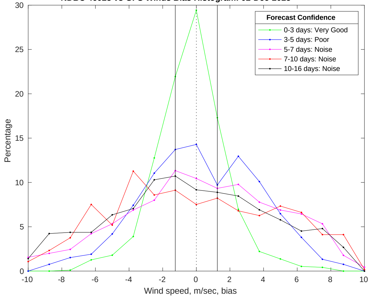
NDBC 46028 vs GFS Winds Bias Histogram: 02-Dec-2025
