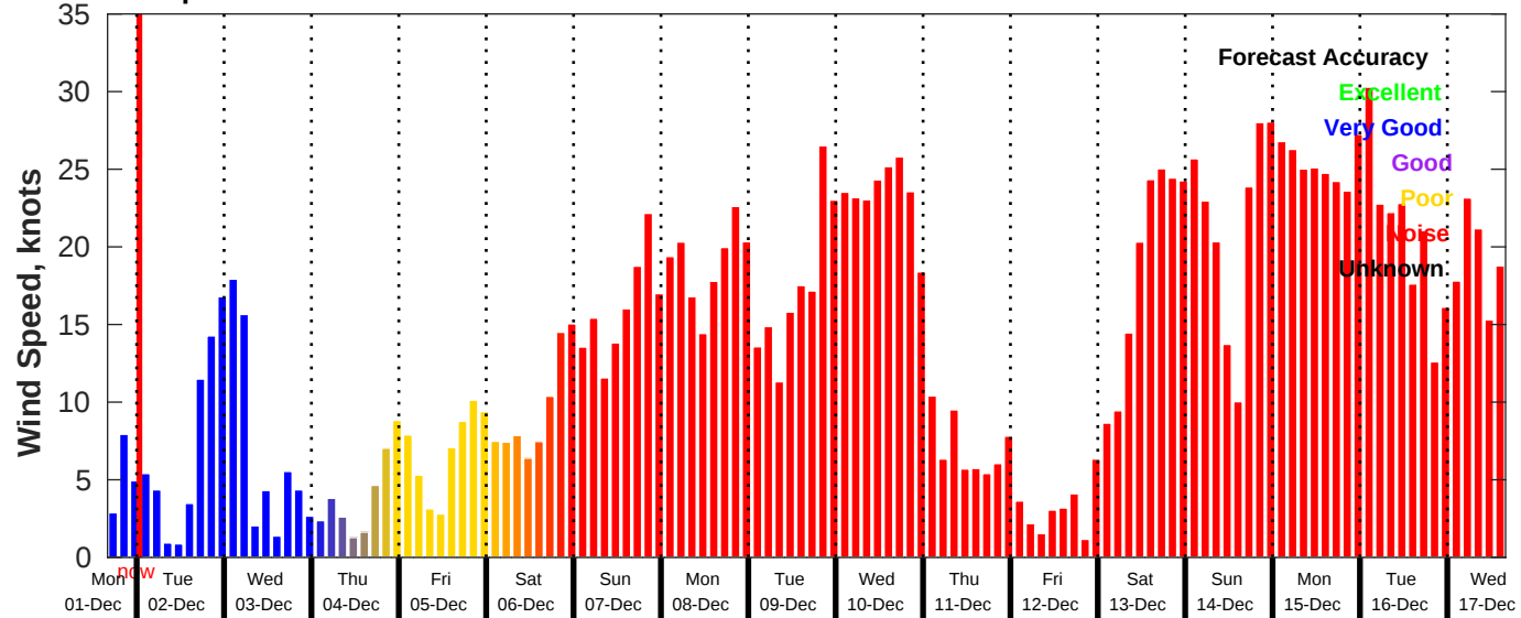
GFS Wind Speed Forecast for NDBC 46028 from 01-Dec-2025 16:00:00 to 17-Dec-2025 16:00:00
