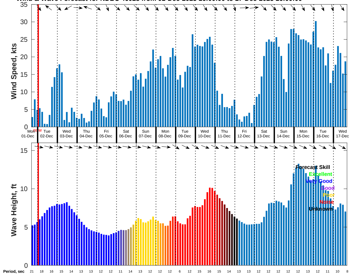
Wind & Wave Forecast for NDBC 46028 from 01-Dec-2025 16:00:00 to 17-Dec-2025 16:00:00
