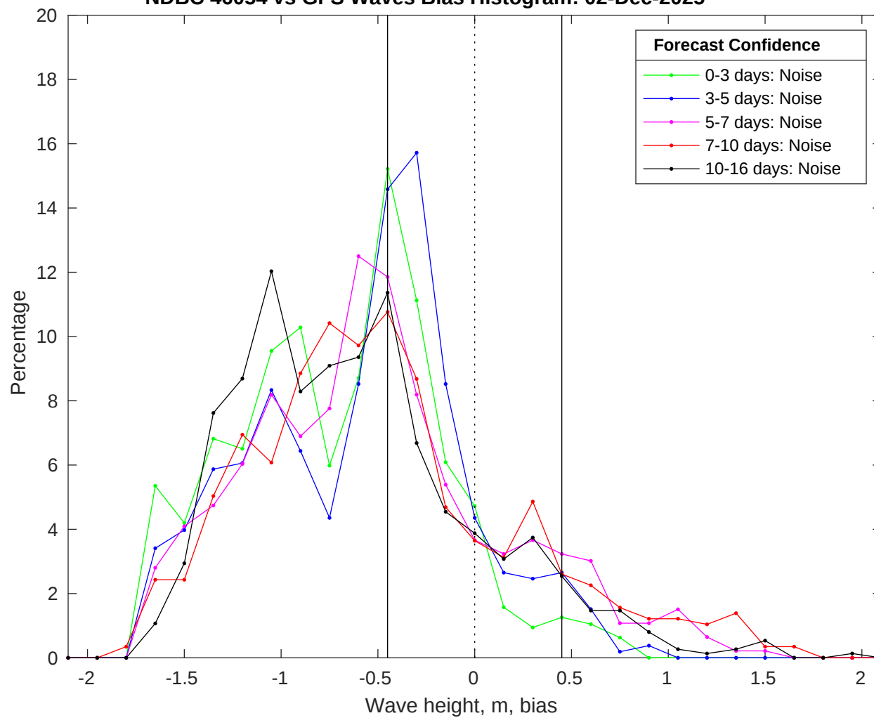
NDBC 46054 vs GFS Waves Bias Histogram: 02-Dec-2025
