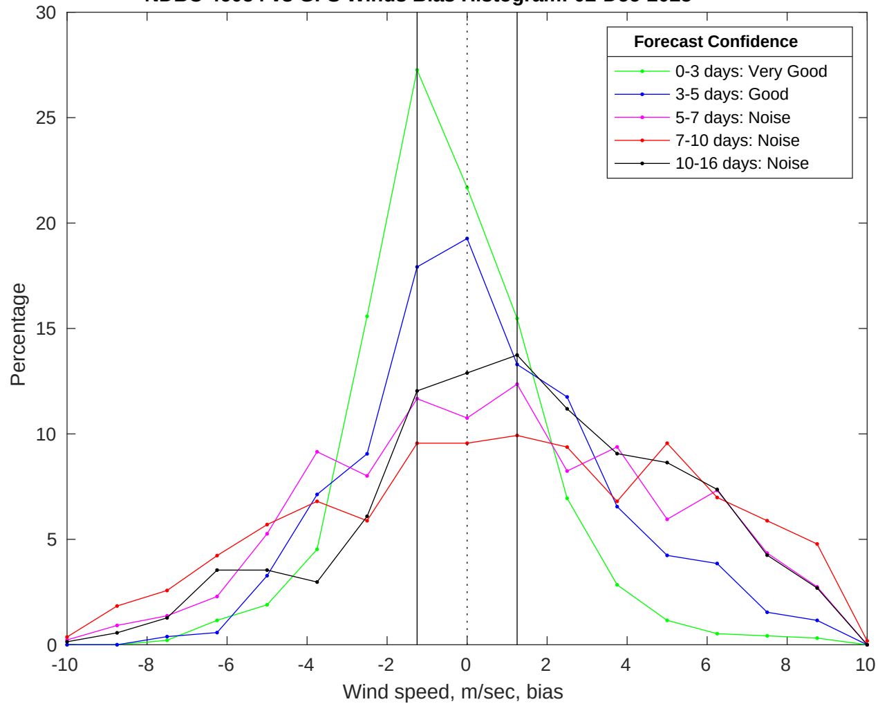
NDBC 46054 vs GFS Winds Bias Histogram: 02-Dec-2025
