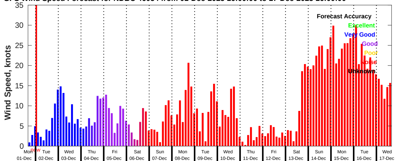
GFS Wind Speed Forecast for NDBC 46054 from 01-Dec-2025 16:00:00 to 17-Dec-2025 16:00:00
