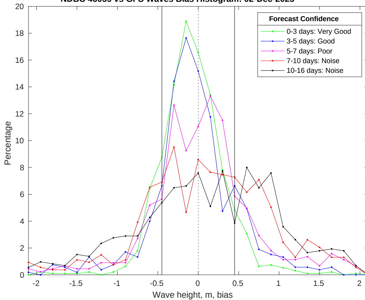
NDBC 46059 vs GFS Waves Bias Histogram: 02-Dec-2025
