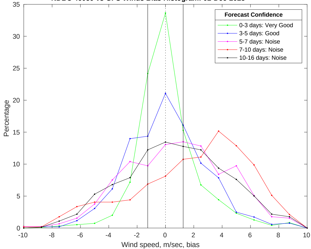
NDBC 46059 vs GFS Winds Bias Histogram: 02-Dec-2025
