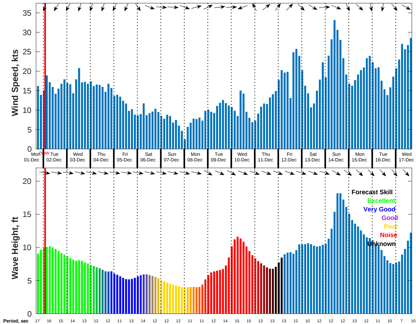
Wind & Wave Forecast for NDBC 46059 from 01-Dec-2025 17:00:00 to 17-Dec-2025 17:00:00
