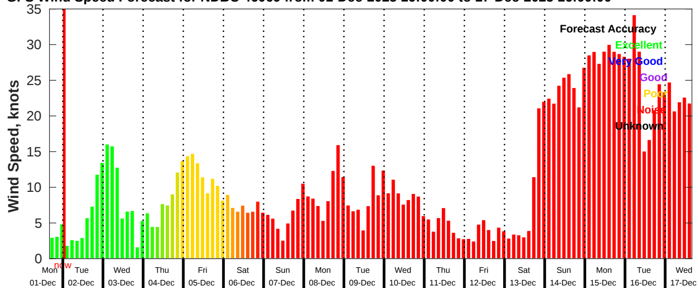
GFS Wind Speed Forecast for NDBC 46069 from 01-Dec-2025 16:00:00 to 17-Dec-2025 16:00:00
