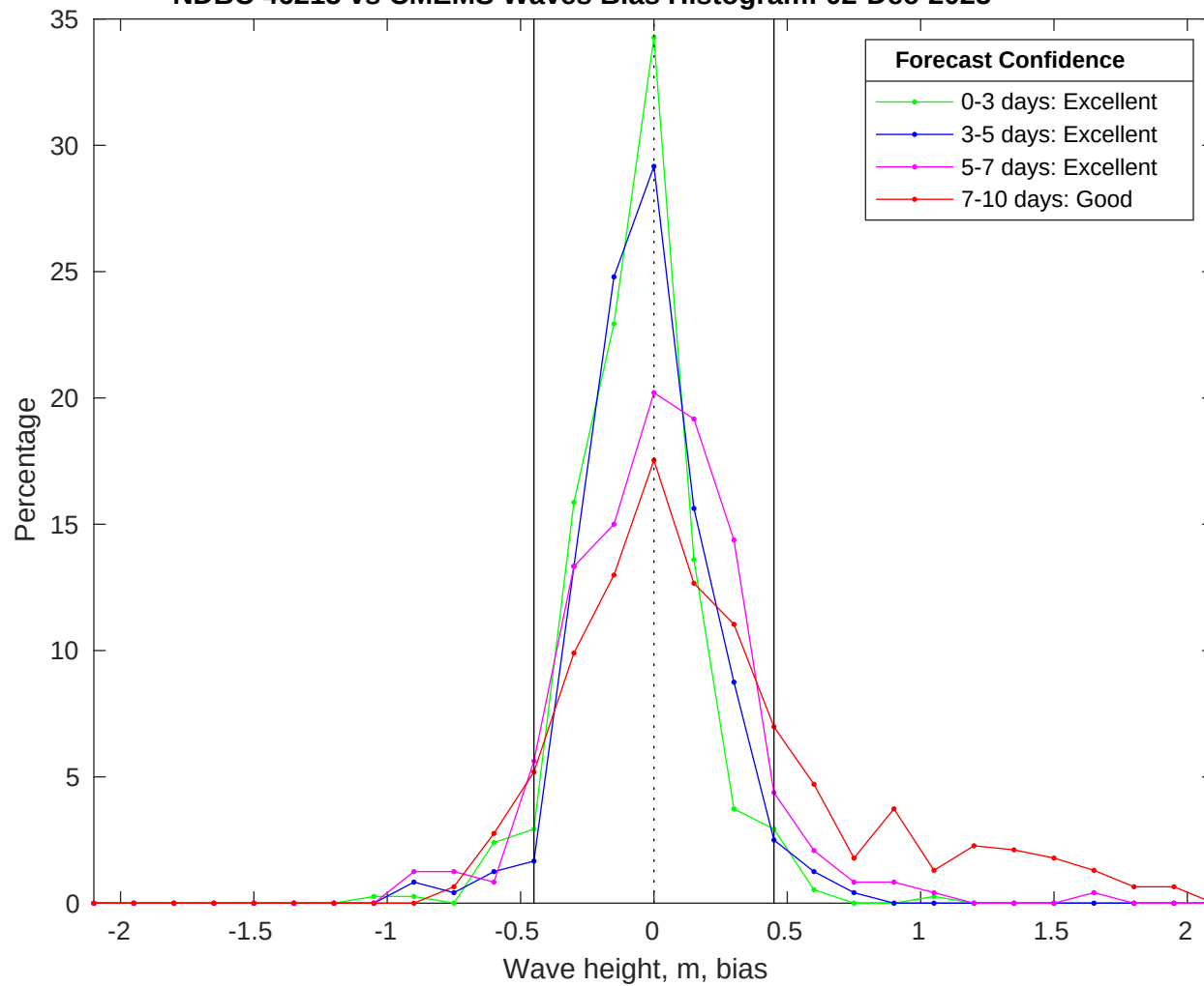
NDBC 46215 vs CMEMS Waves Bias Histogram: 02-Dec-2025
