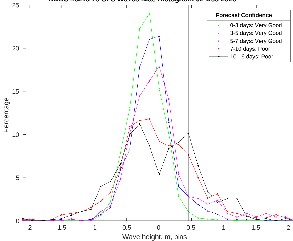
NDBC 46215 vs GFS Waves Bias Histogram: 02-Dec-2025
