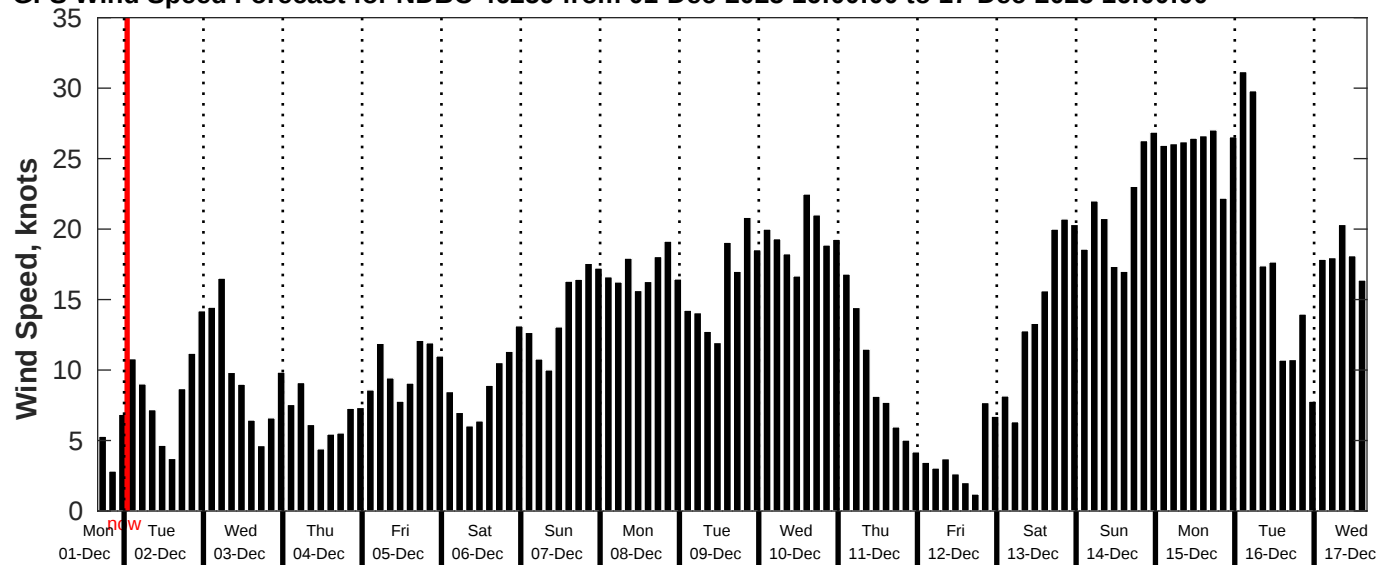
GFS Wind Speed Forecast for NDBC 46259 from 01-Dec-2025 16:00:00 to 17-Dec-2025 16:00:00
