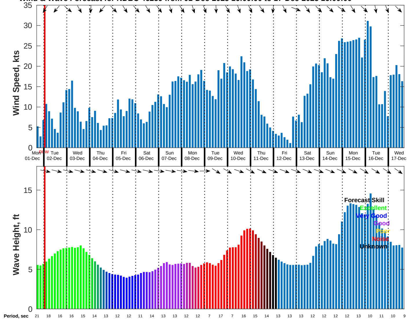
Wind & Wave Forecast for NDBC 46259 from 01-Dec-2025 16:00:00 to 17-Dec-2025 16:00:00
