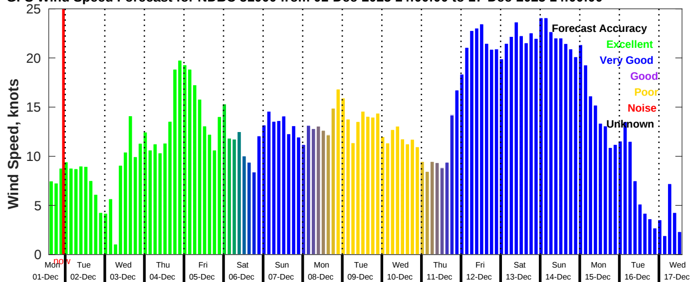
GFS Wind Speed Forecast for NDBC 51000 from 01-Dec-2025 14:00:00 to 17-Dec-2025 14:00:00
