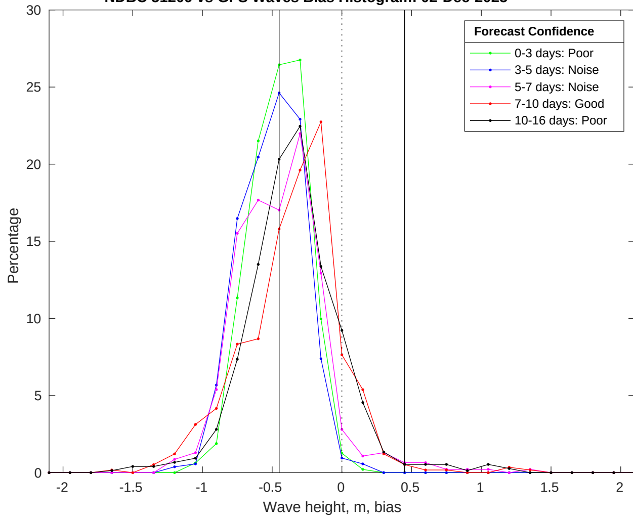
NDBC 51209 vs GFS Waves Bias Histogram: 02-Dec-2025
