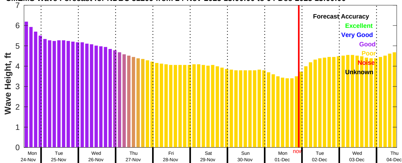
CMEMS Wave Forecast for NDBC 51209 from 24-Nov-2025 13:00:00 to 04-Dec-2025 13:00:00
