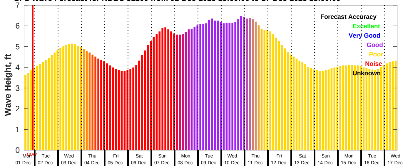
GFS Wave Forecast for NDBC 51209 from 01-Dec-2025 13:00:00 to 17-Dec-2025 13:00:00
