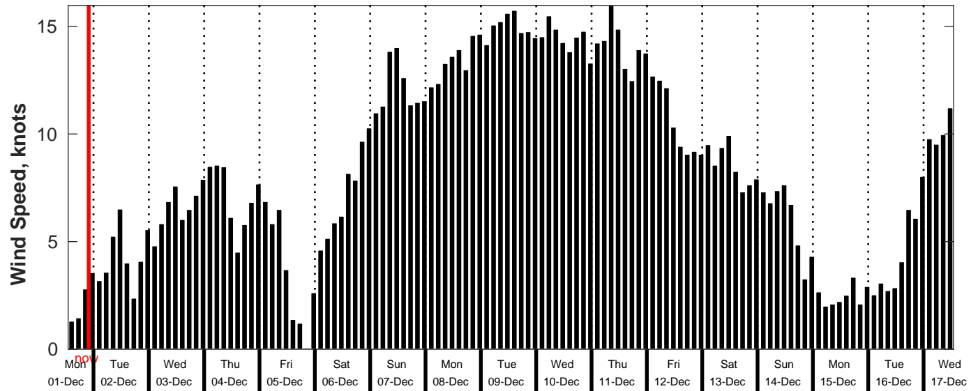
GFS Wind Speed Forecast for NDBC 51209 from 01-Dec-2025 13:00:00 to 17-Dec-2025 13:00:00
