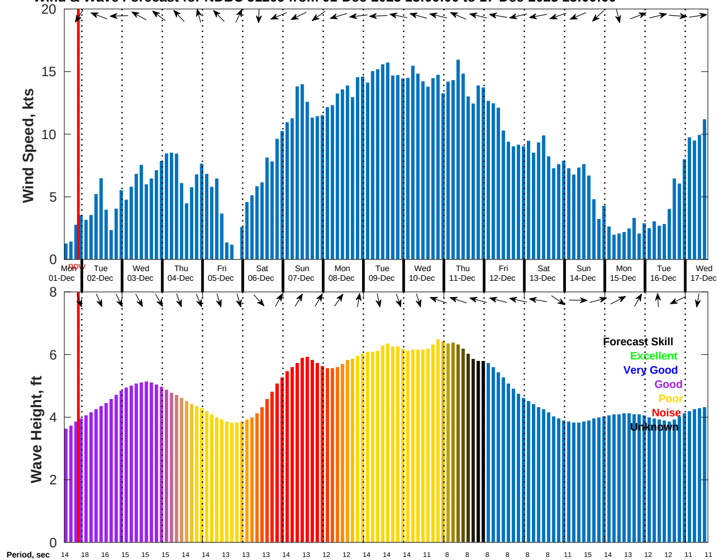
Wind & Wave Forecast for NDBC 51209 from 01-Dec-2025 13:00:00 to 17-Dec-2025 13:00:00
