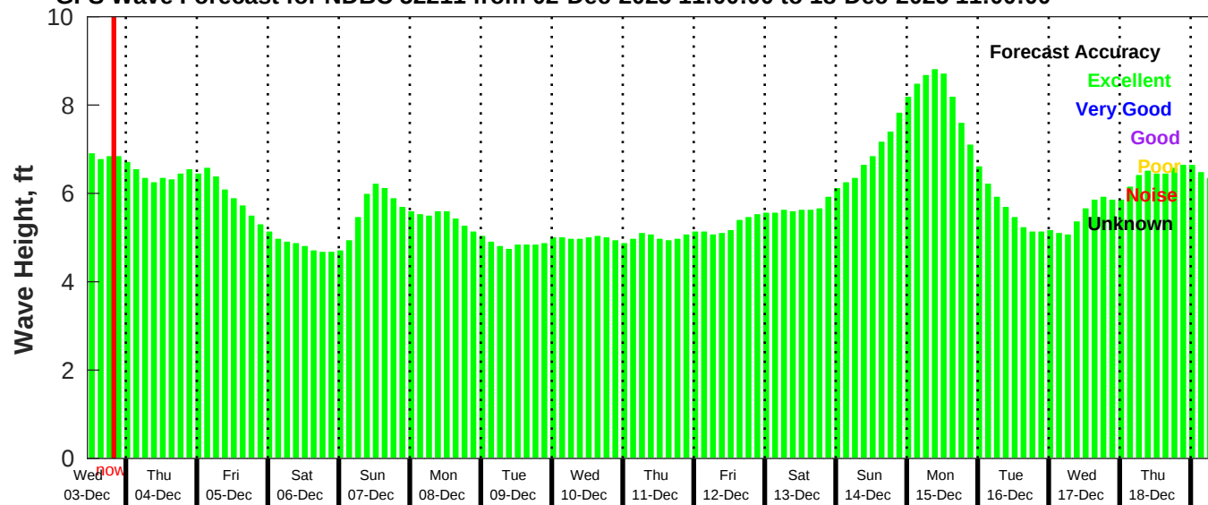
GFS Wave Forecast for NDBC 52211 from 02-Dec-2025 11:00:00 to 18-Dec-2025 11:00:00
