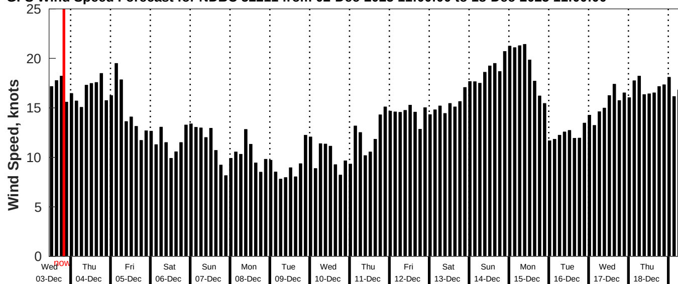
GFS Wind Speed Forecast for NDBC 52211 from 02-Dec-2025 11:00:00 to 18-Dec-2025 11:00:00
