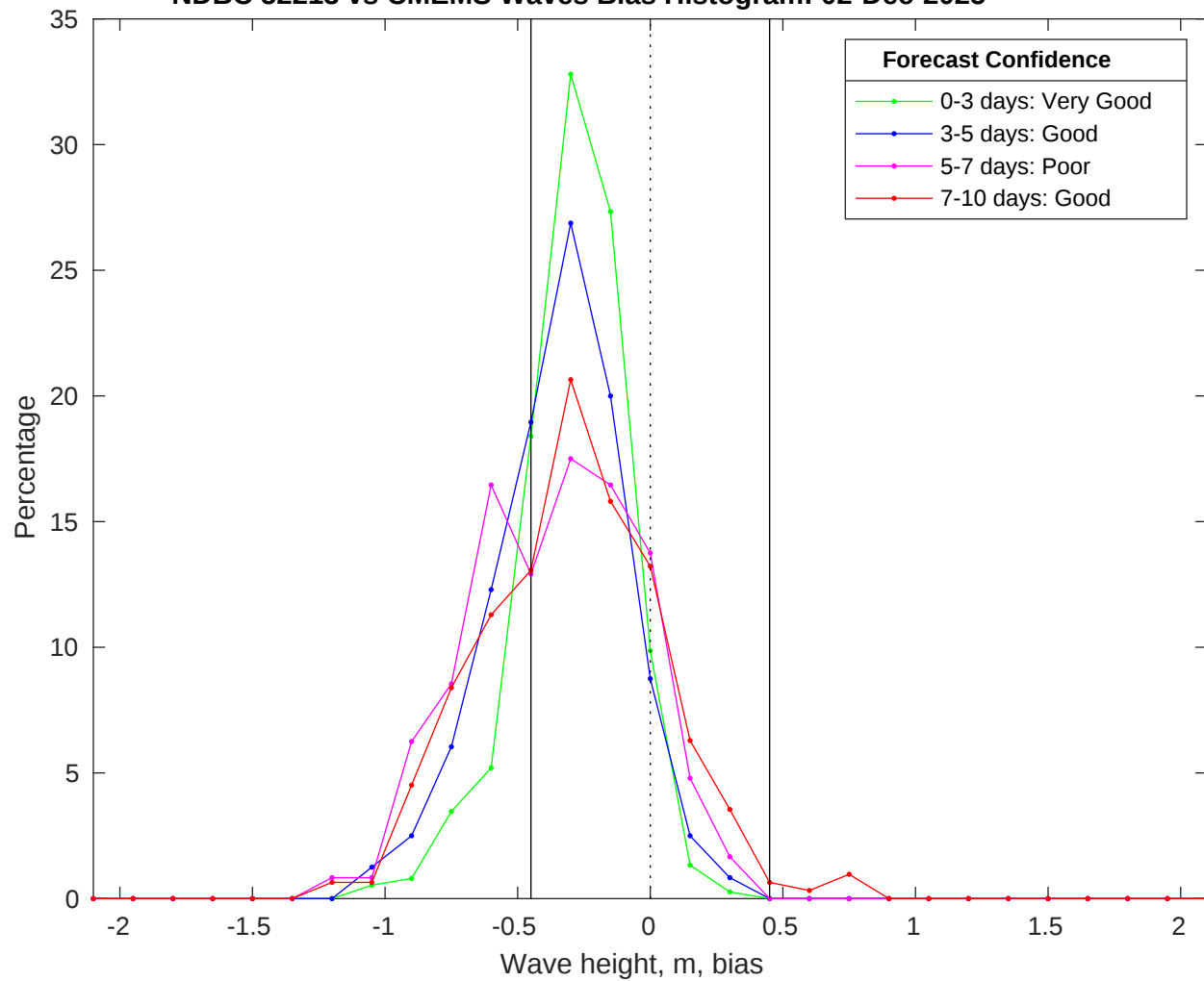
NDBC 52213 vs CMEMS Waves Bias Histogram: 02-Dec-2025
