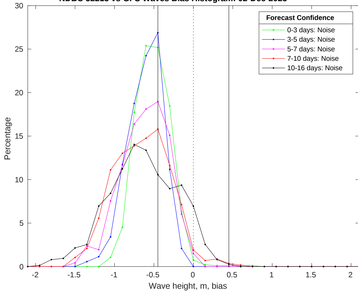
NDBC 52213 vs GFS Waves Bias Histogram: 02-Dec-2025
