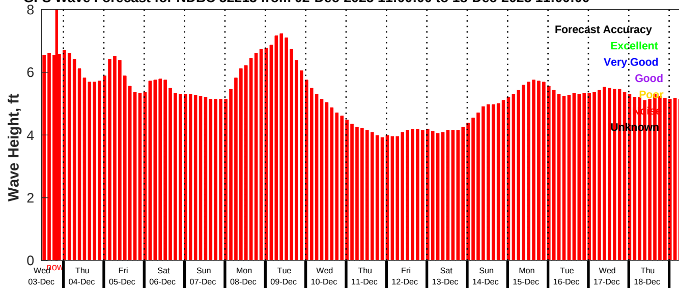
GFS Wave Forecast for NDBC 52213 from 02-Dec-2025 11:00:00 to 18-Dec-2025 11:00:00
