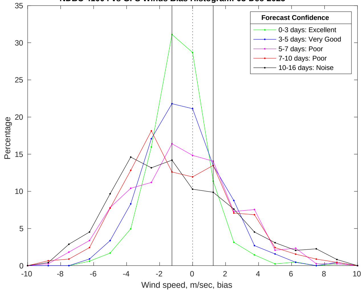
NDBC 41004 vs GFS Winds Bias Histogram: 03-Dec-2025
