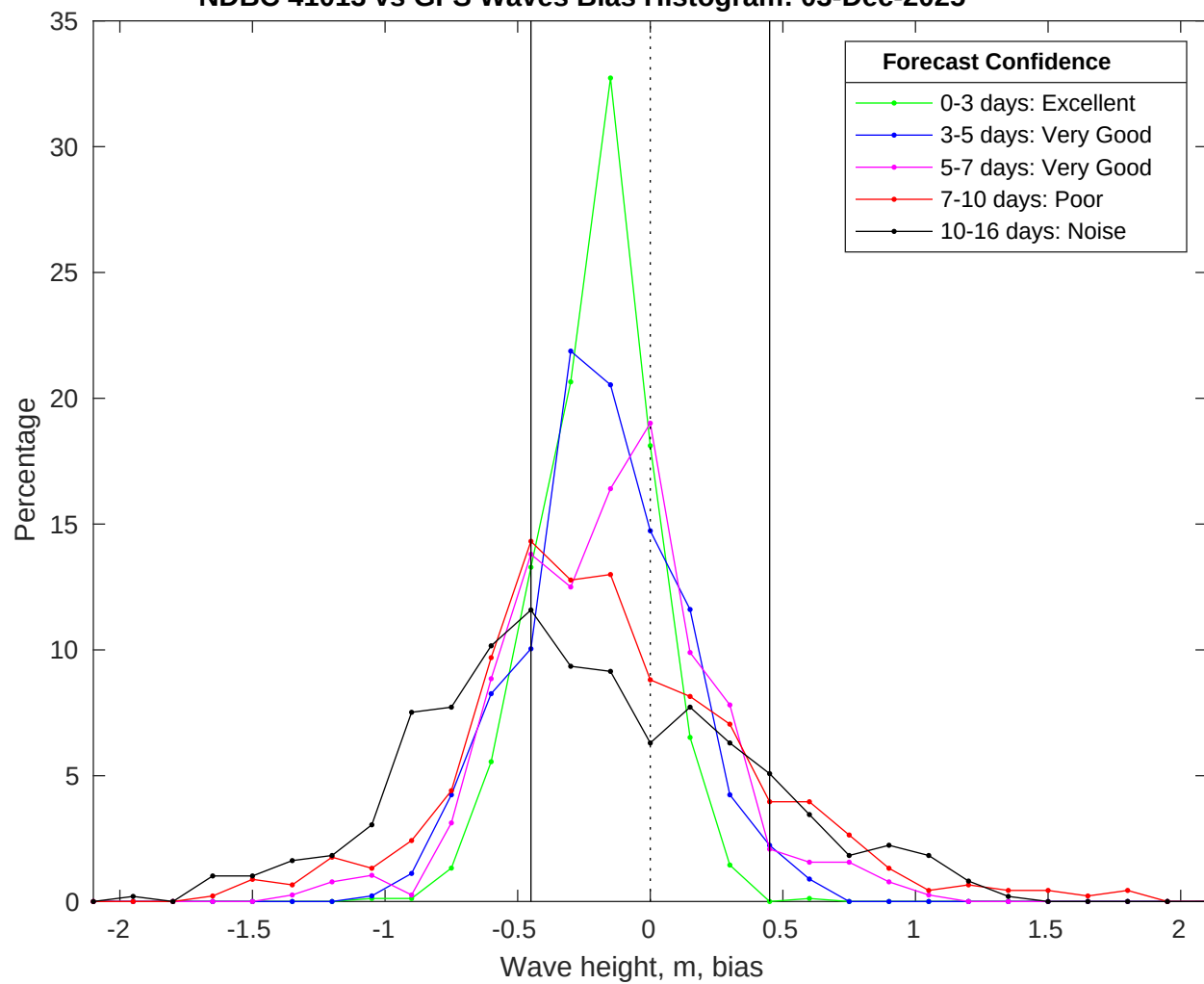
NDBC 41013 vs GFS Waves Bias Histogram: 03-Dec-2025
