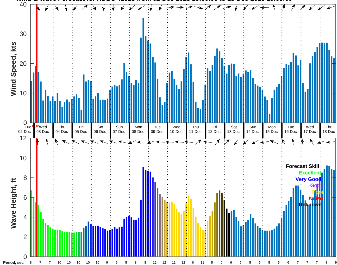
Wind & Wave Forecast for NDBC 41013 from 02-Dec-2025 19:00:00 to 18-Dec-2025 19:00:00
