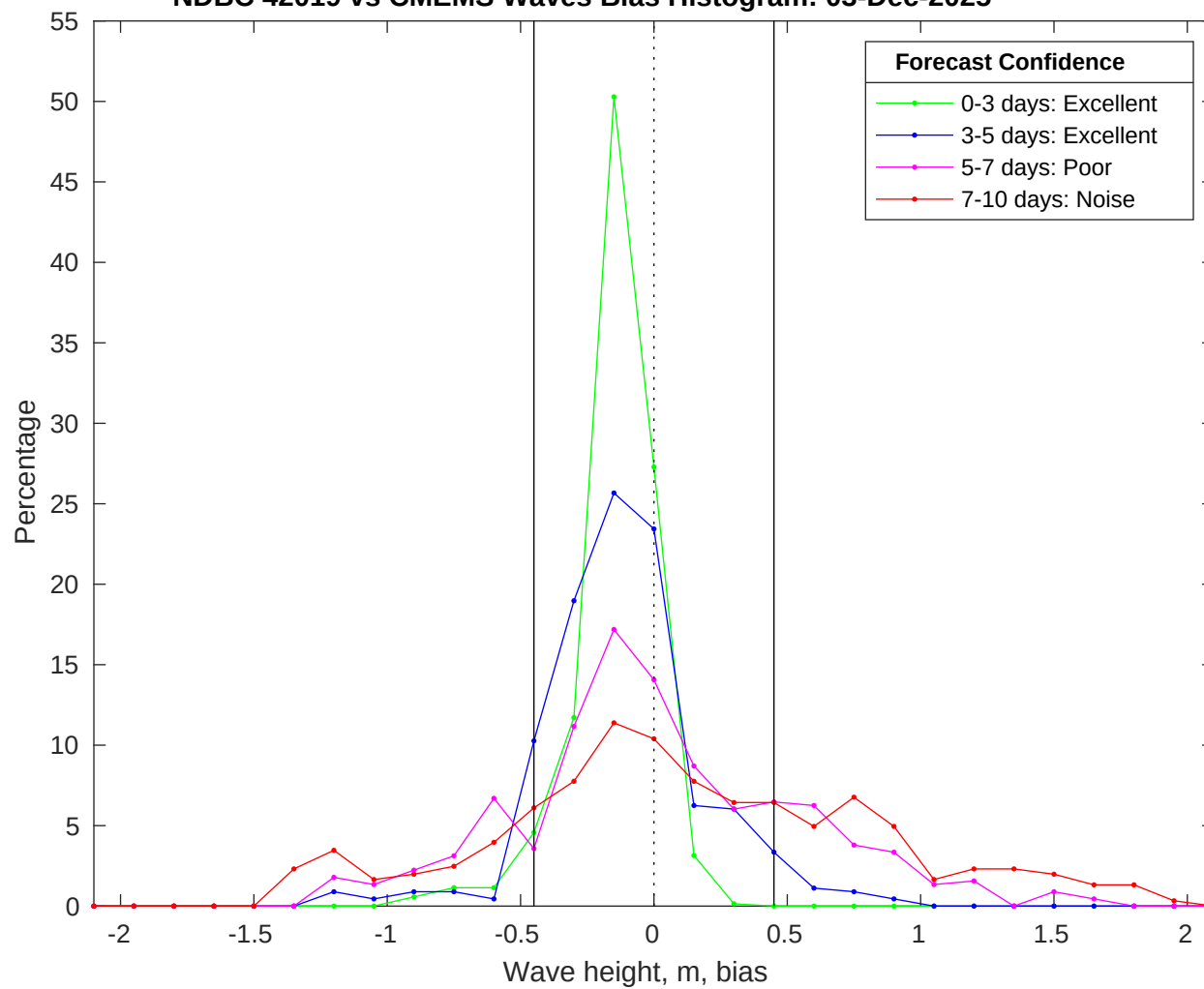
NDBC 42019 vs CMEMS Waves Bias Histogram: 03-Dec-2025
