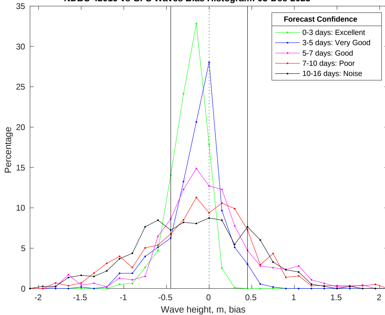
NDBC 42019 vs GFS Waves Bias Histogram: 03-Dec-2025
