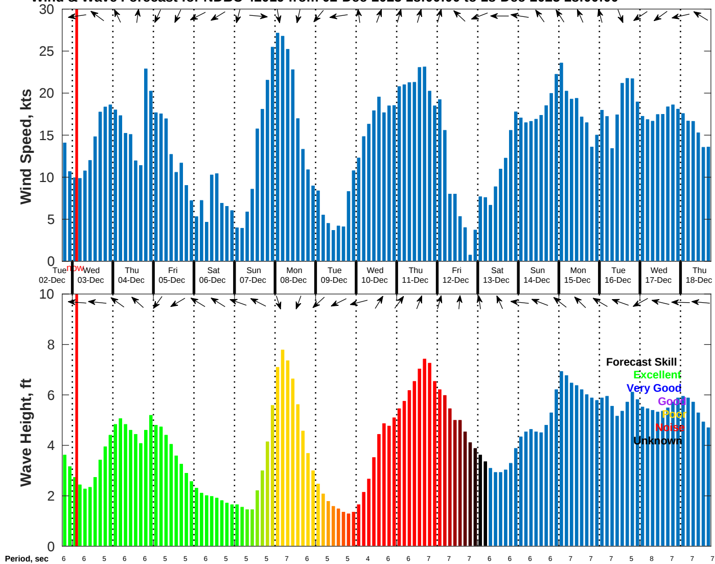
Wind & Wave Forecast for NDBC 42019 from 02-Dec-2025 18:00:00 to 18-Dec-2025 18:00:00
